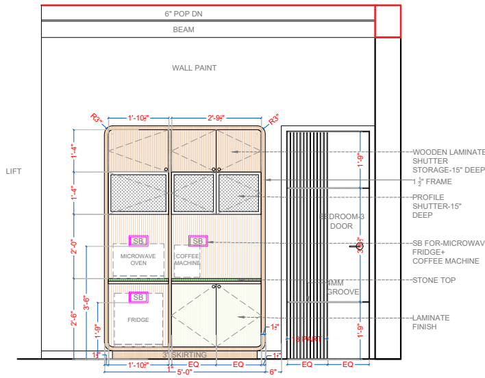
ELEVATION-B
