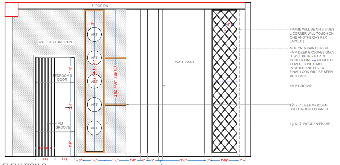
ELEVATION-C
